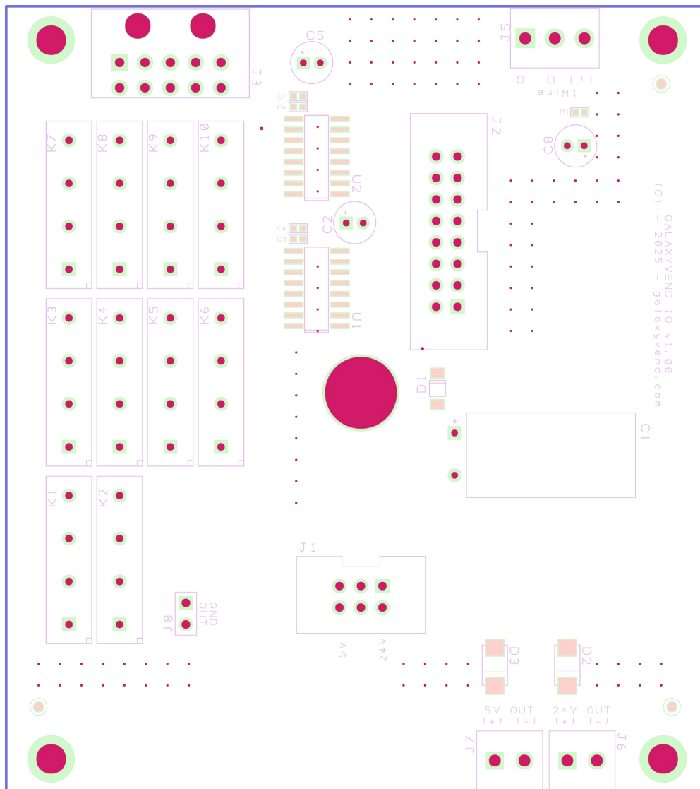
Figure 2: Relays board
