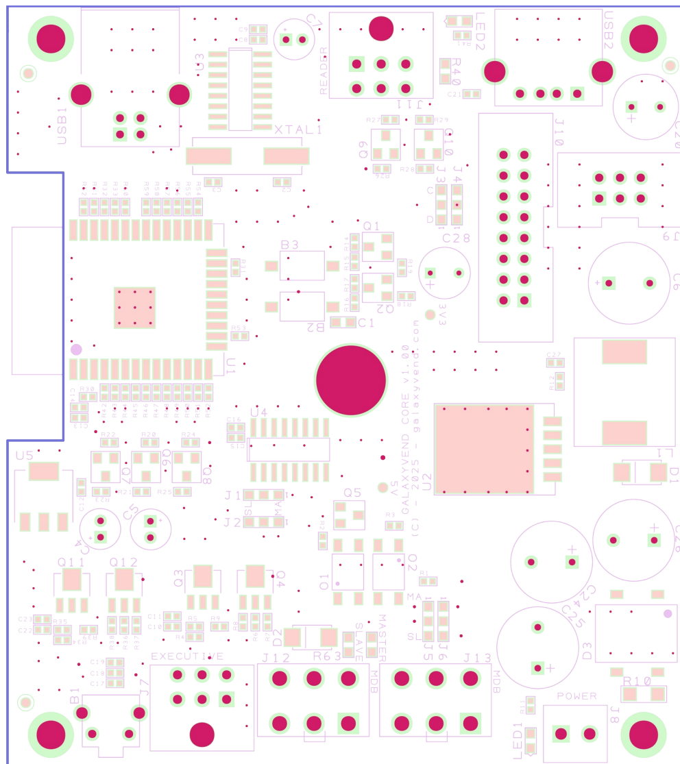
Figure 1: Core board
